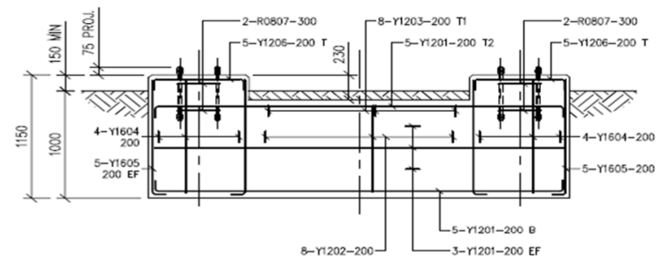
220kV D.S.B. ISOL. SUPPORT BASE 1-SET COMPRISES OF 3 BASES (SEE PLAN VIEW ON ISOL. FOUND. SET)
