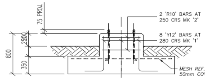
3 (1-SET) - 220kV TRIPLE POLE C.B. SUPPORT BASE' 1-SET COMPRISES OF 3 BASES
